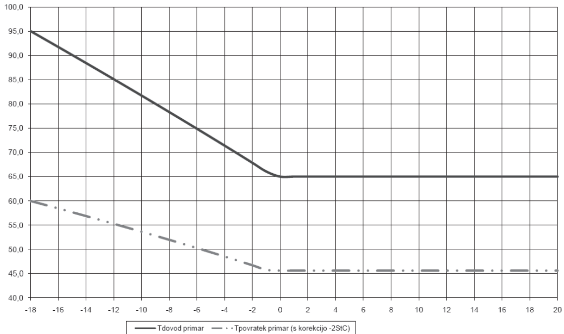
Temperaturni diagram
