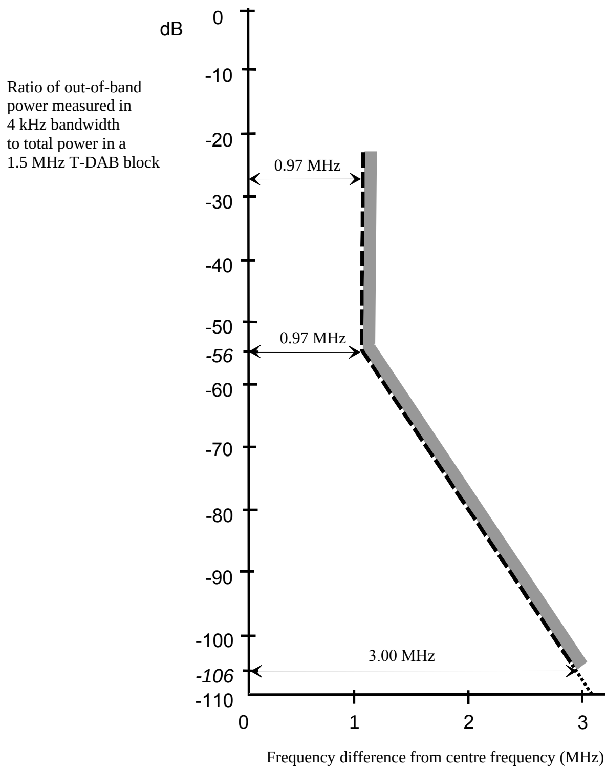
Figure 1: Spectrum mask for T-DAB out-of-band emissions
