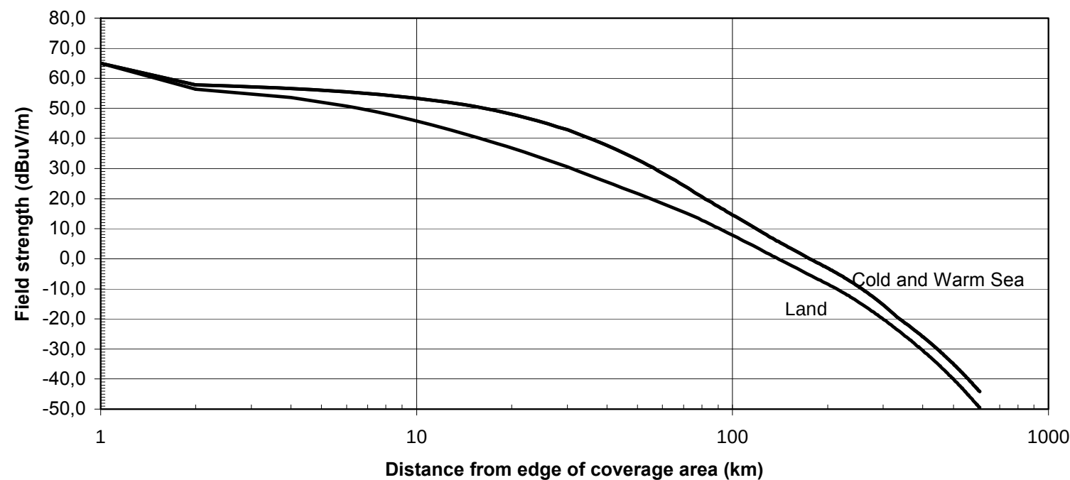
Figure 8a: Interference potential of Reference Network Three for 50 % of time
