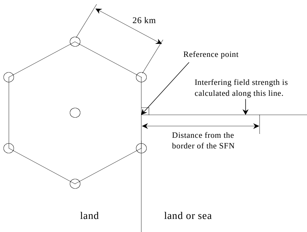
Figure 4: Layout diagram of Reference Network Two
