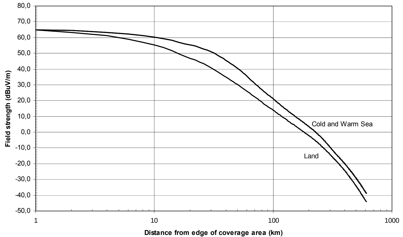
Figure 6a: Interference potential of Reference Network One for 50 % of time
