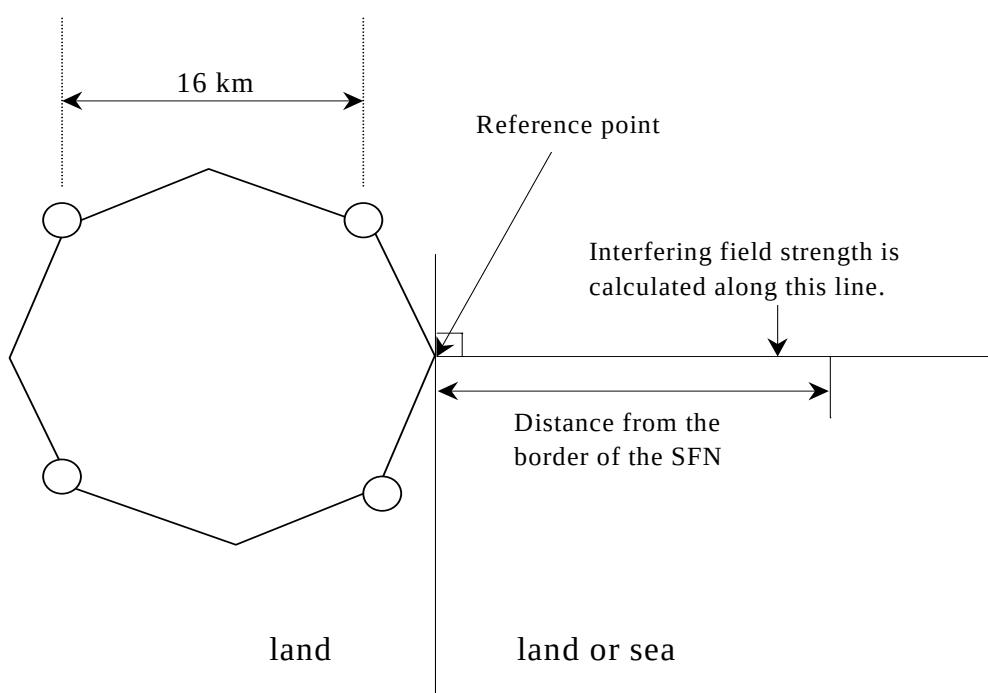
Figure 5: Layout diagram of Reference Network Three.
