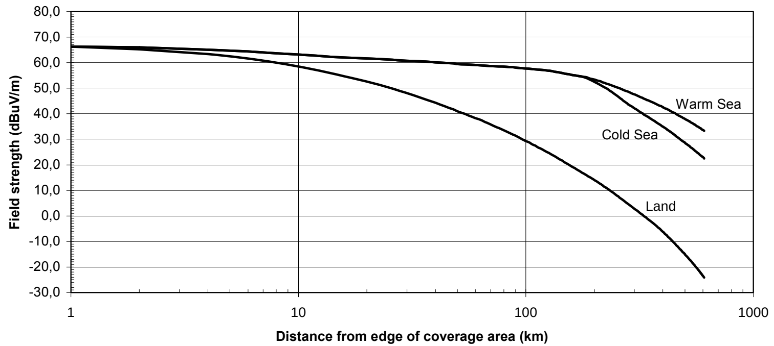
Figure 6b: Interference potential of Reference Network One for 1% of time
