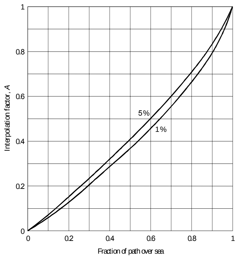
Figure 4 Interpolation for mixed land/sea paths
