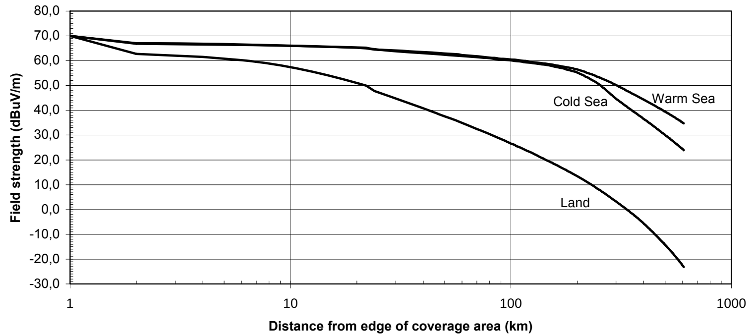
Figure 7b: Interference potential of Reference Network Two for 1% of time
