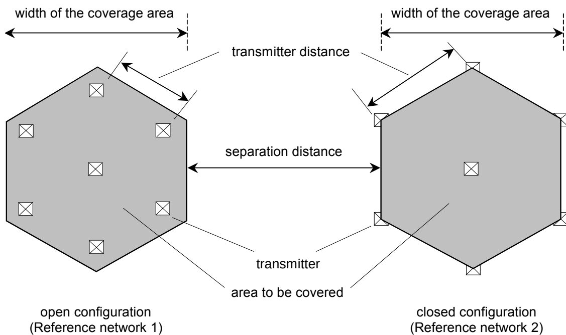
Figure 2: Example of T-DAB network structures and distances – co-block case
