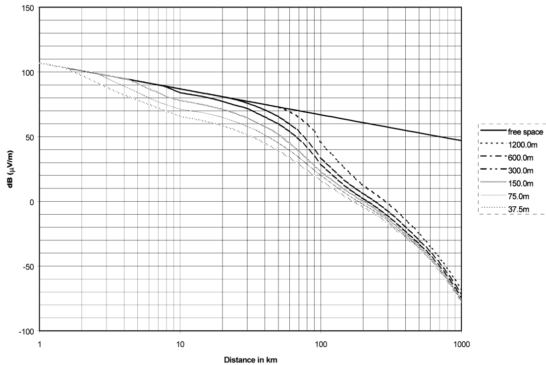
Figure 2a: Field strength for 1 kW e.r.p. versus distance as a function of effective transmitting antenna height; COLD SEA; 50 % of the time
