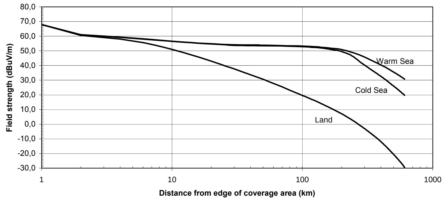
Figure 8b: Interference potential of Reference Network Three for 1% of time
