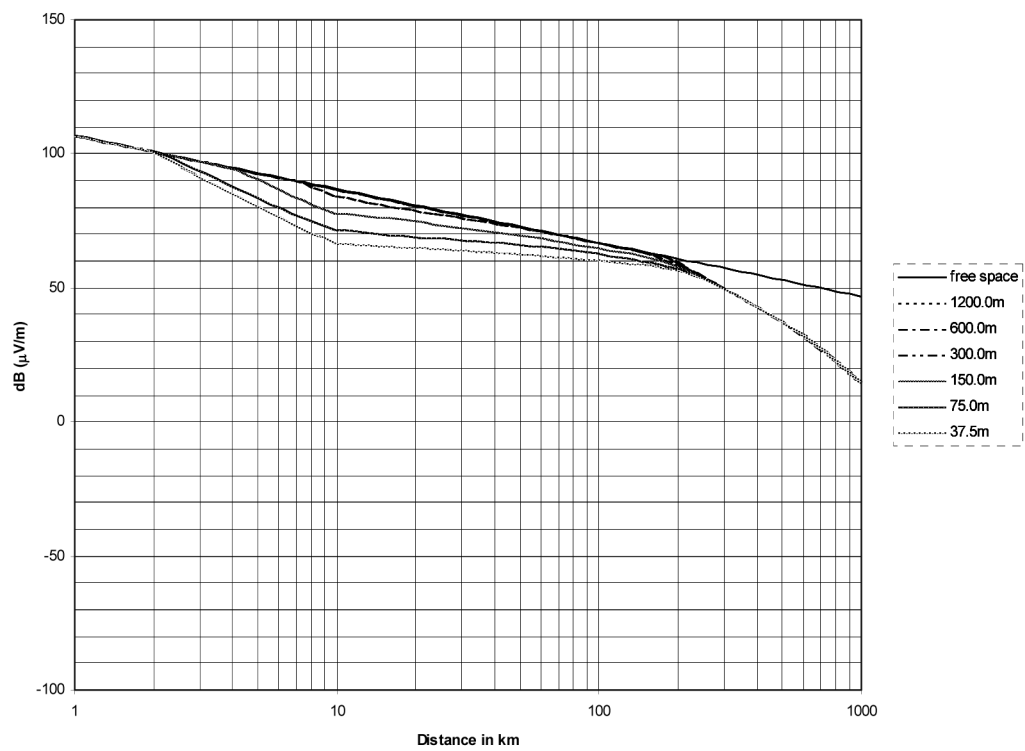
Figure 3b: Field strength for 1 kW e.r.p. versus distance as a function of effective transmitting antenna height; WARM SEA; 1 % of the time
