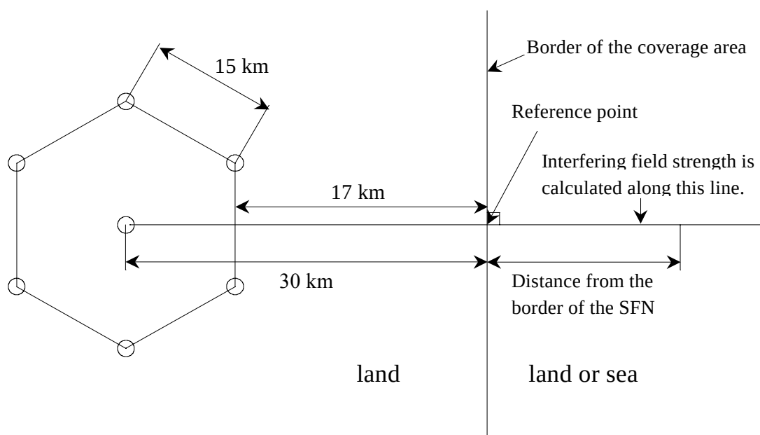
Figure 3: Layout diagram of Reference Network One.
