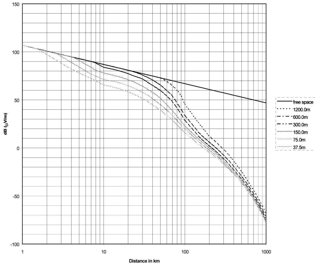
Figure 3b: Field strength for 1 kW e.r.p. versus distance as a function of effective transmitting antenna height; WARM SEA; 1 % of the time
