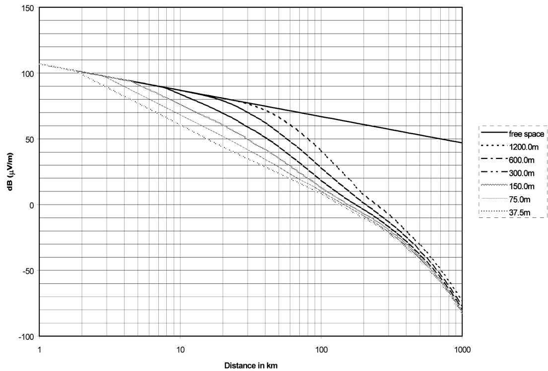
Figure 1a: Field strength for 1 kW e.r.p. versus distance as a function of effective transmitting antenna height; LAND; 50 % of the time
