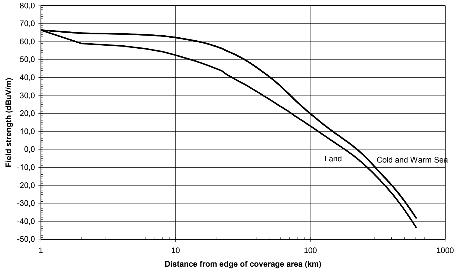
Figure 7a: Interference potential of Reference Network Two for 50 % of time
