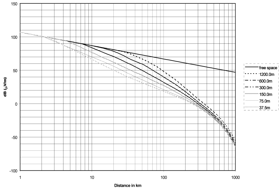
Figure 1b: Field strength for 1 kW e.r.p. versus distance as a function of effective transmitting antenna height; LAND; 1 % of the time
